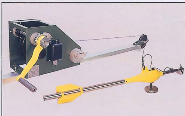
Fig. 7: Cable-suspended current meter with jib, 100 kg single-drum winch, Z 215 counter set and 50 kg middle piece .
